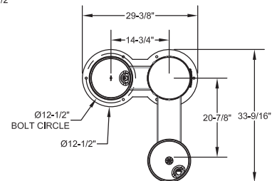
CWBF-3FA-HC-PET & CWBF-3FA-CHD-PET (REAR PET LOCATION)
