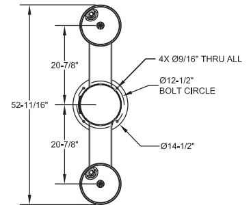
ROUGH-IN HC AND SAH
