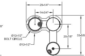
REAR PET ROUGH-IN
