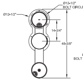
SIDE PET ROUGH-IN
